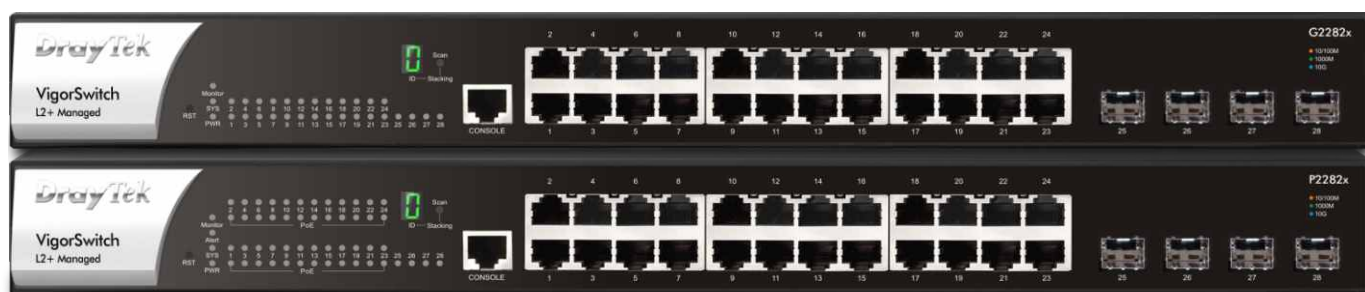
↑ Console Port ↑ 24x Gigabit Ethernet ↑ 4x SFP+ Ports
