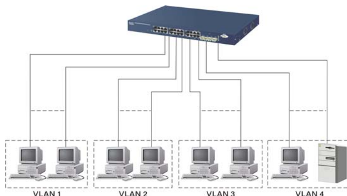
Fig. 2-4 Port-based VLAN Diagram
