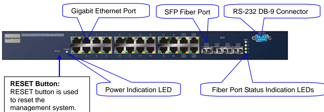
Fig. 1-2 Front View of GEL2P-SW24
