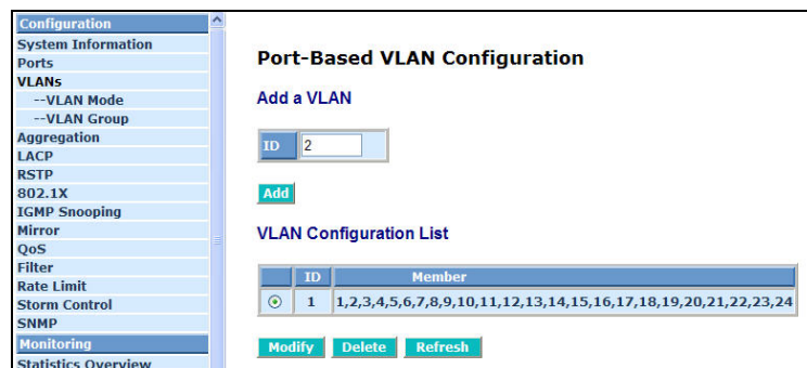
Fig. 4-7 Port-Based VLAN Configuration
