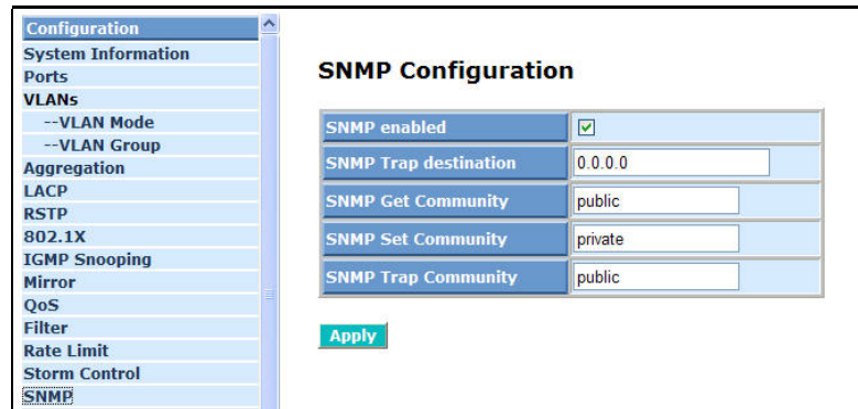
Fig. 4-27 SNMP Configuration
